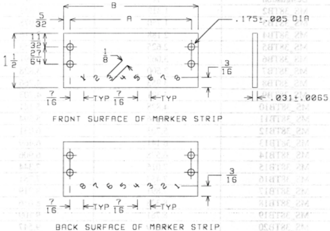
Figure 1. Terminal Board Marker Strip, Type MSA38TB8.
