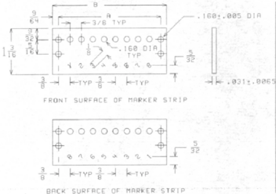
Figure 1. Terminal Board Marker Strip, Type MSA40TB8.
